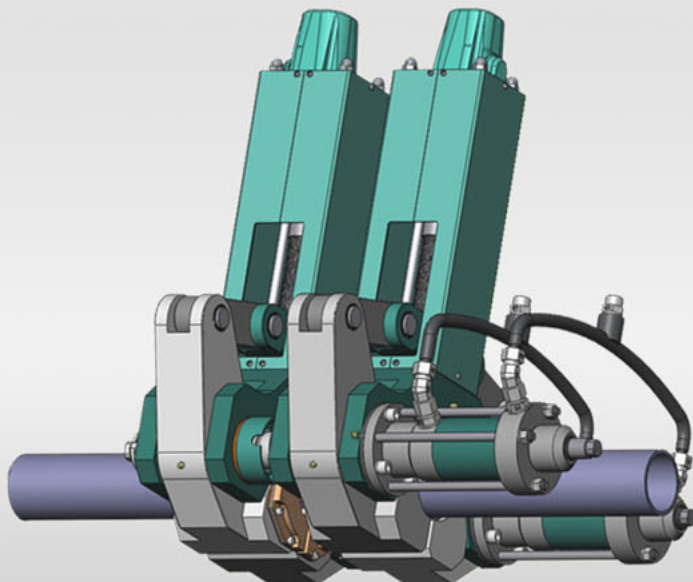
MODEL MD200 (Motor Actuator)
